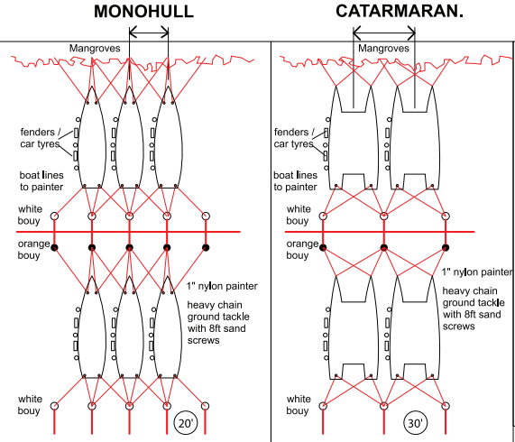
Typical mooring arrangement
